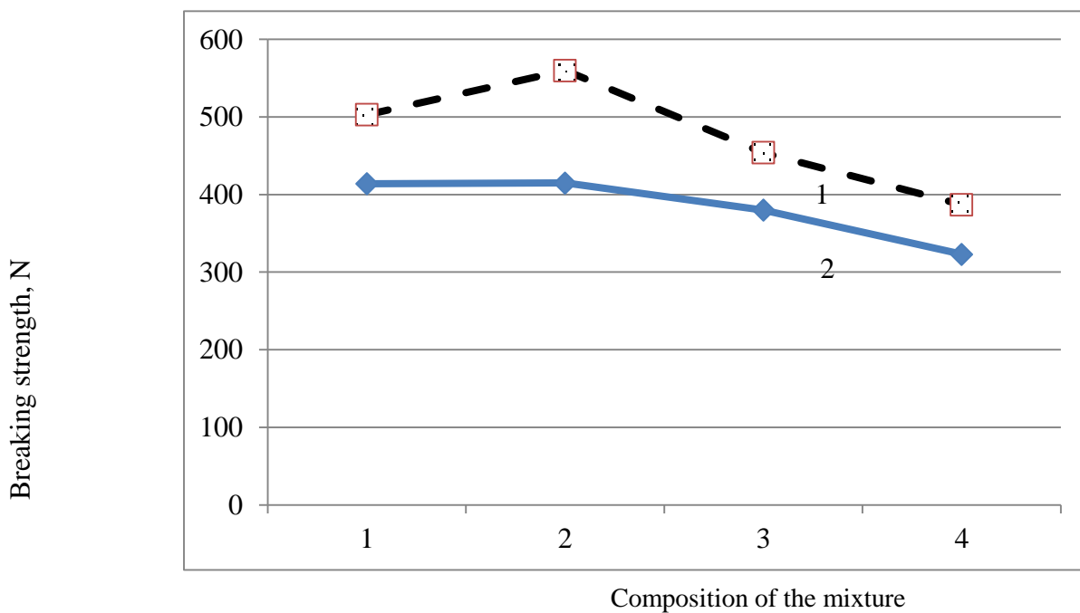
Figure 2. Variation of the tensile strength of the yarn obtained from a mixture of different composition and processed fibers in the warp and weft direction.
