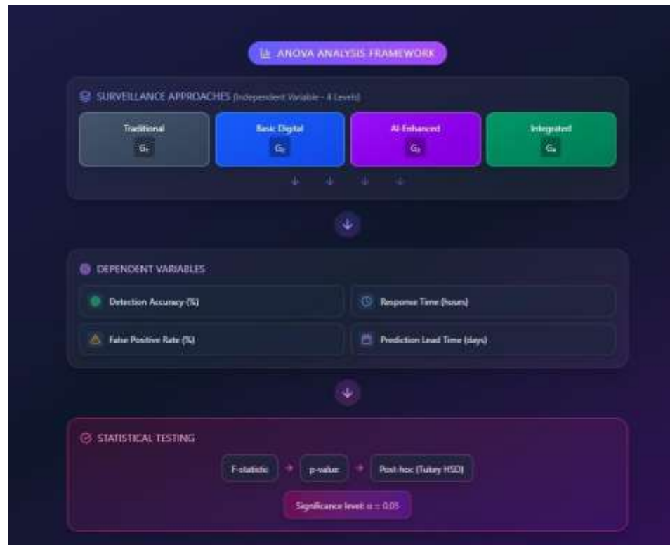
Figure 6. ANOVA Analysis Framework
