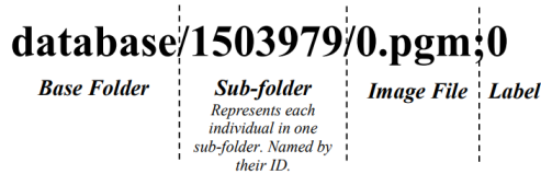
Fig 5 : Content Structure in SQL QUERY File
